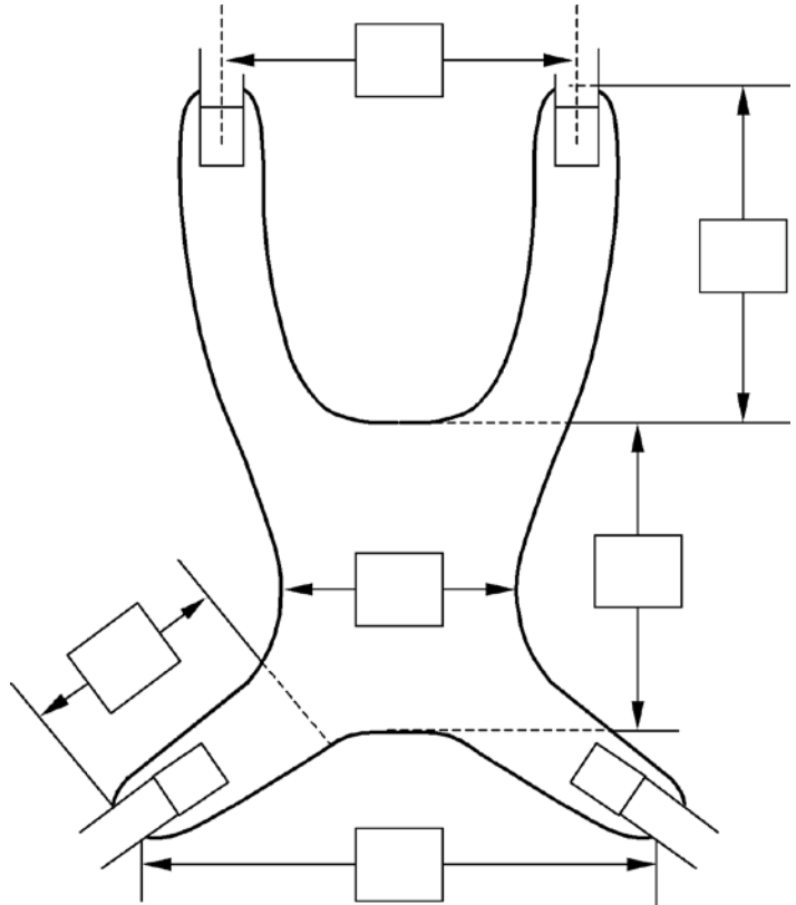
Chest harness
